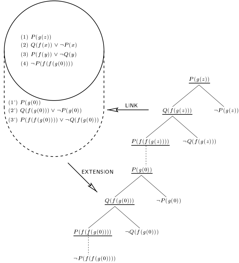
Figure 1: Hyper-tableau derivation for Ex. 1.
