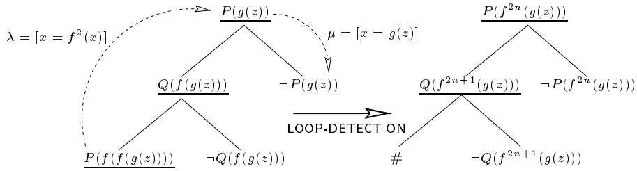
Figure 2: Loop-detection for Ex. 1.
